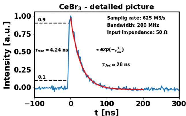
Figure 2. A close up view of one pulse, which was recorded by the \text{CeBr}_3 scintillation detector. Maximal pulse height was normalized to one.
