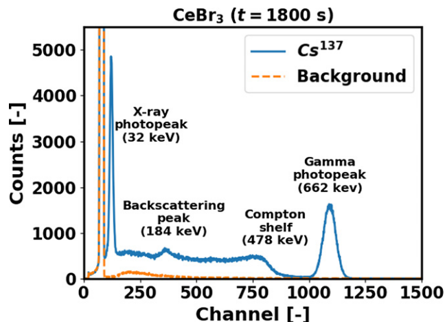
Figure 3. The gamma-ray spectrum of ^{137}\text{Cs} recorded by the \text{CeBr}_3 scintillation detector, where all characteristic features of spectra are displayed.
