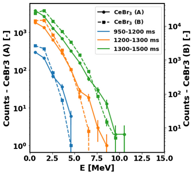
Figure 8. Comparison of HXR energy spectra acquired by two \text{CeBr}_3 spectrometers, where one of spectrometers ( \text{CeBr}_3(\text{A}) ) was inside lead shielding with the wall thickness of 5 cm. Another one ( \text{CeBr}_3(\text{B}) ) was unshielded.
