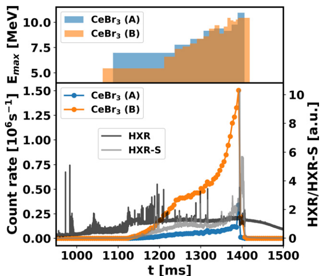
Figure 7. Comparison of signals from standard HXR diagnostic at the COMPASS and newly installed \text{CeBr}_3 spectrometers. Upper sub-figure shows evolution of maximal energy of detected HXR radiation.
