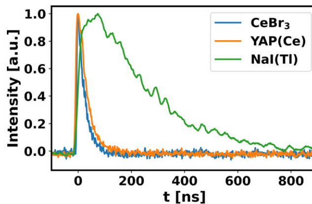
Figure 1. Comparison of pulses with normalized height recorded by various scintillation detectors.
