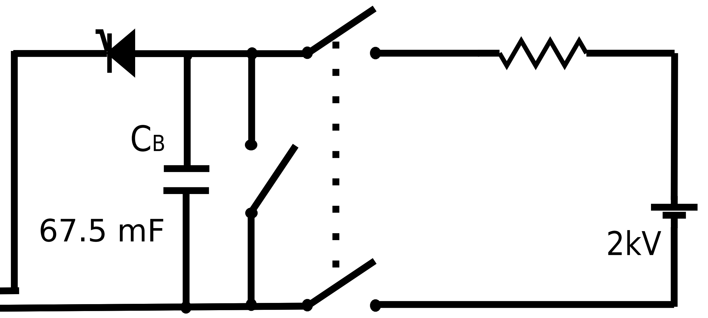
Toroidal magnetic field
