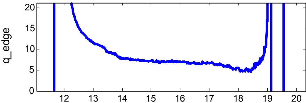
Safety factor on plasma edge in shot 8382
