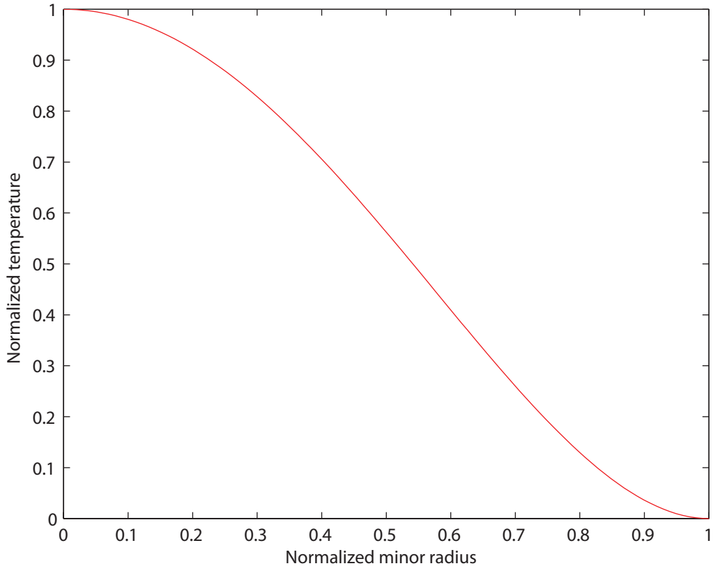
Polynomial temperature profile
