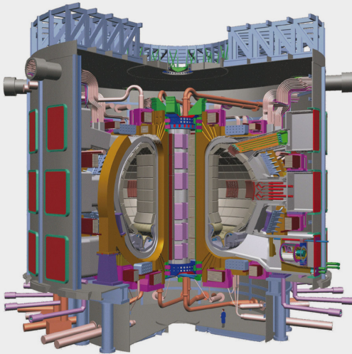
/// Figure 2. General view of the ITER experiment
