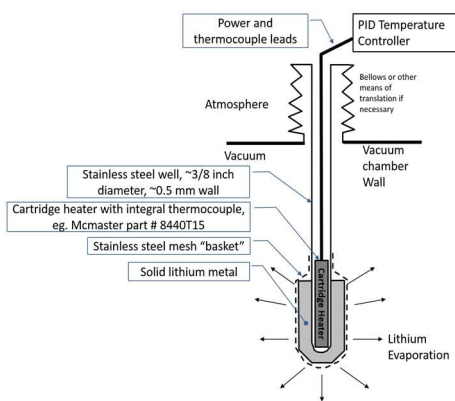
Figure 1. Lithium evaporator schematic.
