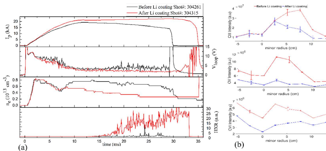
Figure 23. STOR-M plasma discharge parameters before (black line) and after (red line) Li coating (a). The intensity profiles of C III , O V and C VI before (red line) and after (blue line) Li coating (b).
