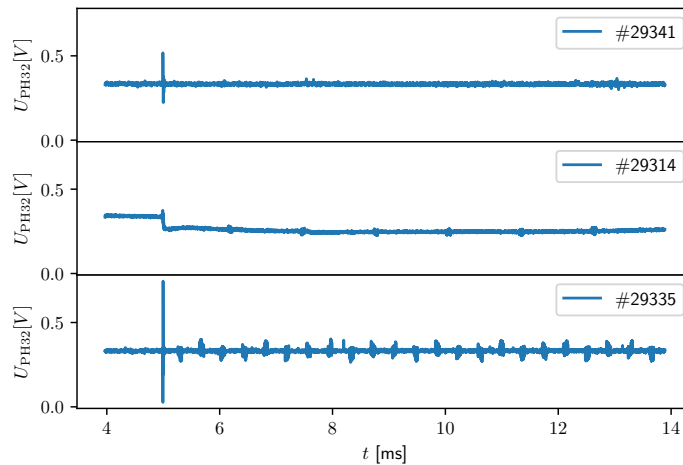
Figure 7. Detected noise. First plot shows peak created by the magnetic field ramp up. The second and third plot show by reading the data by SURE with 1090 \mu s long shutter (shot 29314) and 200 \mu s long shutter (shot 29335).
