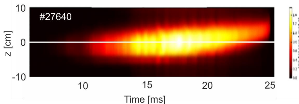
Figure 3. Temporal evolution emission measured by the array of bolometers viewing the plasma vertically from the horizontal port (#27640).
