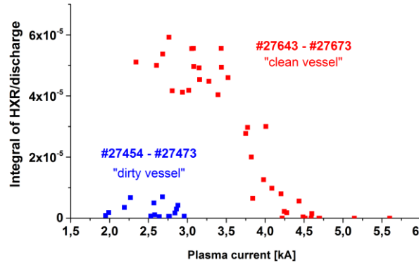
Figure 13. Time integral of HXR versus plasma current for “clean” and “dirty” vessel.
