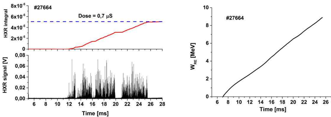
Figure 12. Left - Evolution of the HXR signal (bottom panel) and its time integral (top panel). Right – Maximum energy of RE. #27664 (“clean” vessel).
