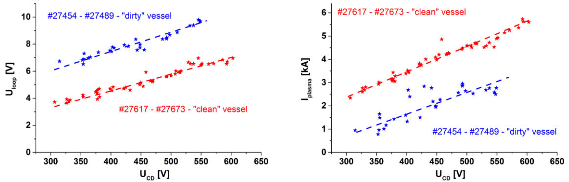
Figure 9. Mean plasma current and the mean loop voltage versus the “real” charging voltage U_{CD} – for “clean” (red symbols) and “dirty” (blue symbols) vessel.
