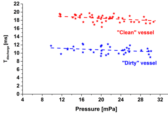
Figure 7. Duration of a discharge versus the pressure of the working gas for “clean” and “dirty” vessel plotted for all values of the charging voltage of the condenser bank used for powering the primary winding of the GOLEM transformer, U_{CD} .
