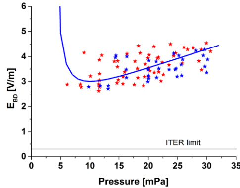
Figure 6. Paschen diagram on GOLEM – for “clean” (red symbols) and “dirty” (blue symbols) vessel for all measured values of U_{CD} . Blue line – model Paschen law.
