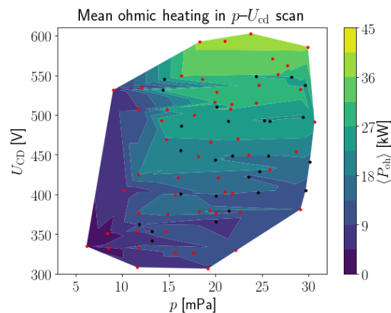
Figure 10. 2D plot of the mean Ohmic power at different pressures and charging voltages U_{CD} for “clean” (red points) “dirty” (black points) vessel.
