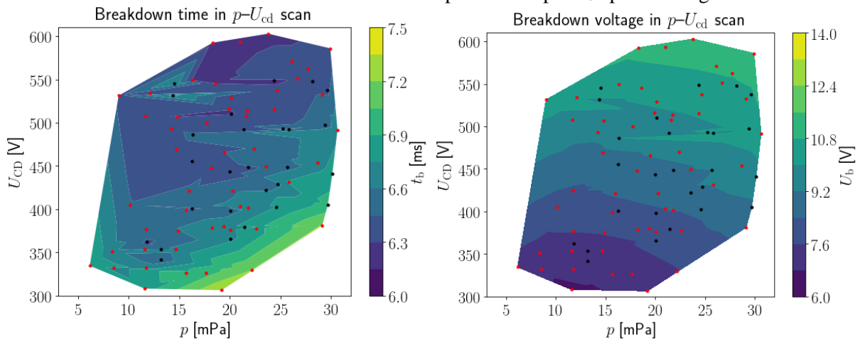
Figure 5. 2D plots in the plane of the pressure and the charging voltages U_{CD} . Red symbols – “clean” vessel, black symbols – “dirty” vessel. Left - the breakdown time, right – the loop voltage at the breakdown.
