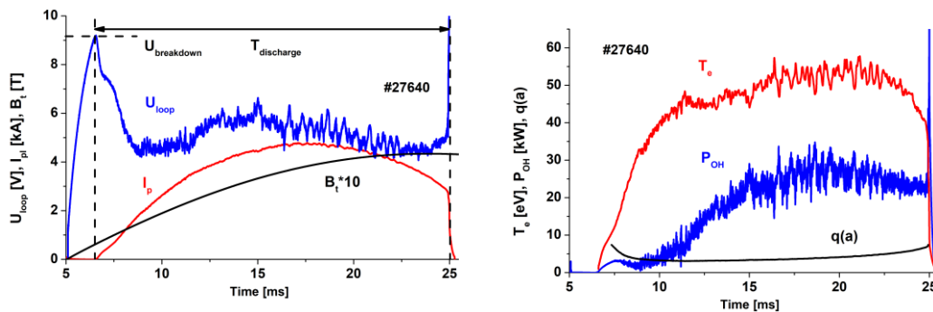
Figure 2. Temporal evolution of the discharge #27640, p = 23.5 mPa, U_{CD} = 400 V – "clean" vessel.
