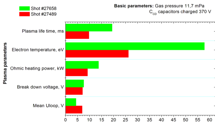
Figure 14. Summary comparison of plasma performance with “dirty vessel” (#27489) and “clean vessel” (#27658).
