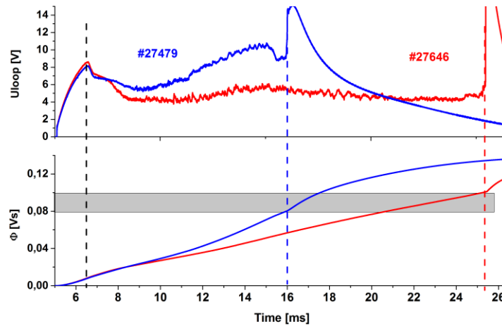
Figure 8. Evolution of the loop voltage and the consumed magnetic flux in the GOLEM transformer for “clean” (red) and “dirty” (blue) vessel.
