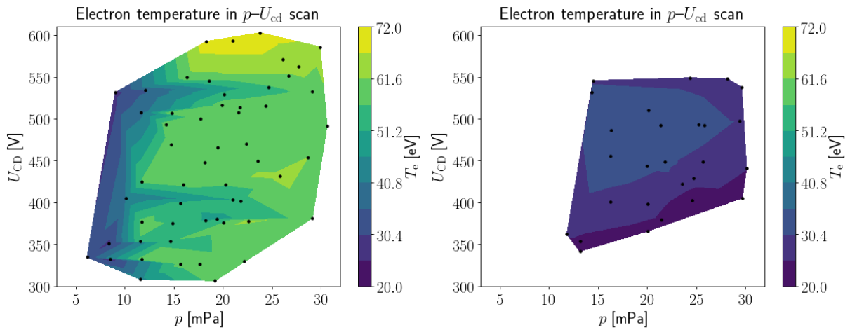
Figure 11. 2D plot of the mean electron temperature at different pressures and charging voltages U_{CD} . Left – “clean” vessel, Right – “dirty” vessel.
