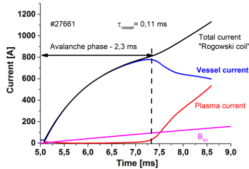
Figure 4. Evolution of the start-up phase on GOLEM.
