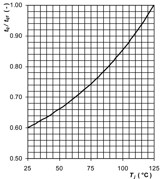
Fig. 12 Normalised maximum turn-off time vs. junction temperature
