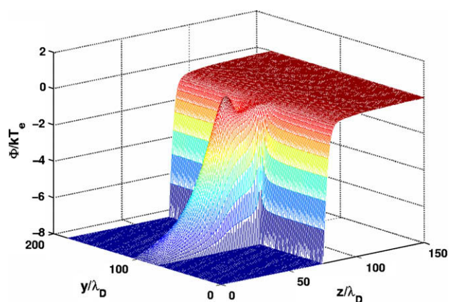
Fig. 7. Computed electric potential normalized to kT_e in a poloidal gap between two tiles for \alpha_{\text{PG}} = 45^\circ .
