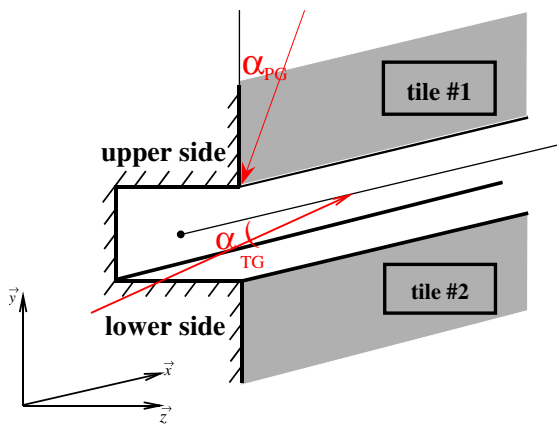
Fig. 3. Schematic view of both toroidal ( \alpha_{TC} ) and poloidal ( \alpha_{PG} ) orientations of the gap with respect to the magnetic field lines.
