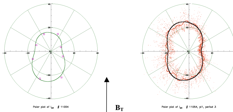
Figure 2. Polar diagrams of the ion saturation current as measured in the same shot by the IGP (left) and the RMP (right) located inside the separatrix ( r= 70 mm). The experimental points are fitted to the KD model [2] (solid lines). #11054 .
