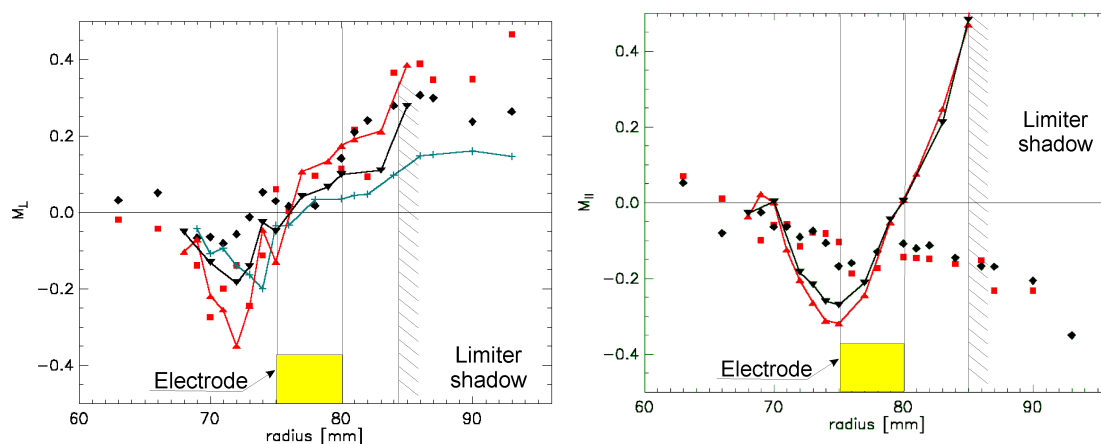
Figure 3. Radial profiles of perpendicular and parallel Mach numbers during electrode biasing as measured simultaneously by the RMP and the IGP. Electrode occupies the range of radii 75-80 mm, i.e. separatrix biasing with U_b = 150 V. Radial profile of the E \times B velocity is shown for comparison in the left panel. Probe data are processed by two methods (denoted as KD [2] and VG [5]). #11027-51.
