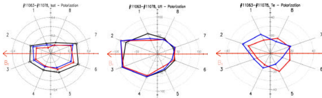
Figure 4. Polar diagrams of the swept IGP. From left to right: Ion saturation current, floating potential, electron temperature. M_{\perp} = -0.23 , M_{\parallel} \sim 0 .
