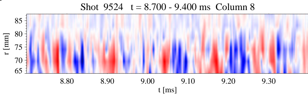
Fig. 3: Signals from upstream column of probes.
