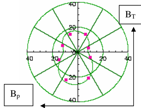
Figure 16. Polar diagram of the ion saturation current measured by individual segments (red squares)
