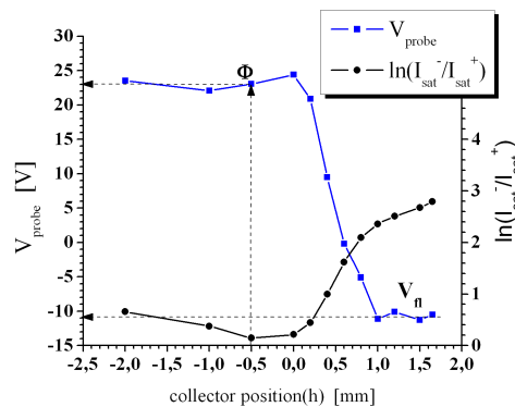
Figure 14. Variation of the collector potential and the logarithm of the R on the collector position
