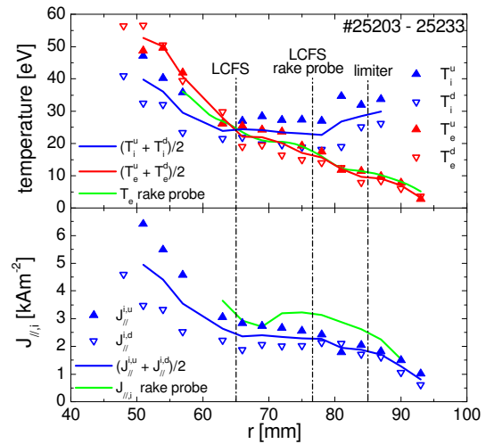
Figure 12. Radial profiles of the electron and ion temperatures (top) and parallel ion saturation current density (bottom) obtained by the STP. T_e and J_{||} are compared with the ones measured by the rake probe.
