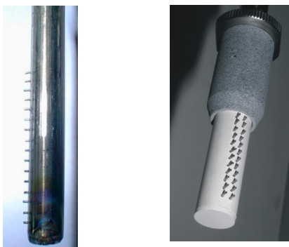
Figure 1. Pictures of the single (left) and the double (right) rake probe.
