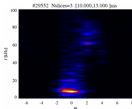
Figure 8. Frequency of magnetic oscillations versus the poloidal mode number m during the biasing period of a discharge.
