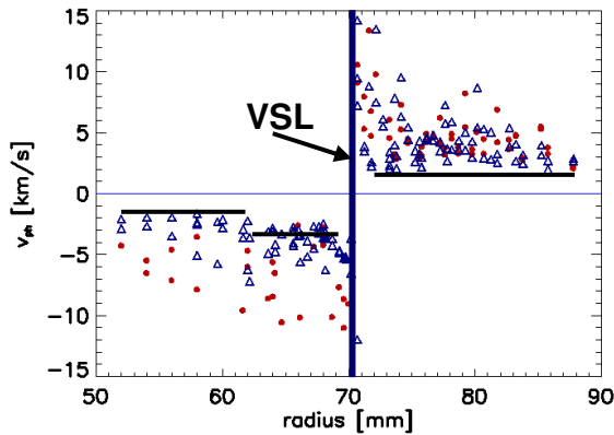
Figure 5. Radial profile of the phase velocity of V_{fl} (red circles) and I_{sat} (blue triangles) fluctuations. The three horizontal lines represent the quantity -\nabla V_{fl}/B_T , which is a minimum estimate of the value of the radial electric field at the given range of radii.
