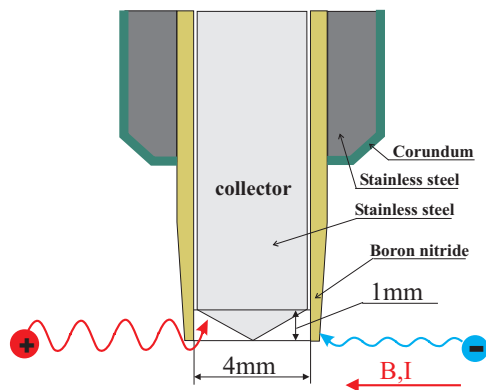
Figure 13. Schematic drawing of the ball-pen probe
