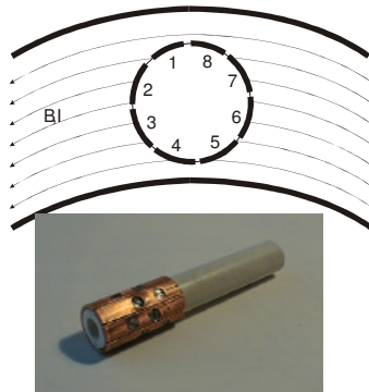
Figure 15. Layout of the Gundestrup probe on the CASTOR. View from the top of the torus
