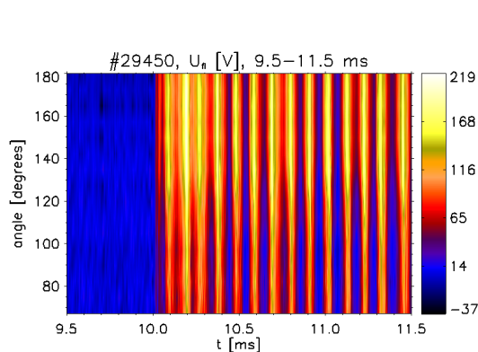
Figure 7. Temporal evolution of the poloidal distribution of V_{||} at the beginning of the biasing period.
