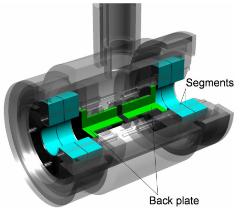
Figure 11. Schematic drawing of the probe head of the STP. Two segmented tunnels are mounted back-to-back in a Mach probe arrangement.
