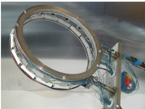
Figure 6. Picture of the full poloidal ring of 96 Langmuir probes. Probes are located at the radius r = 85 mm and their mutual poloidal distance is 5.5 mm. The ring is equipped by 16 Mirnov coils and by 16 Hall sensors to measure the plasma position and to investigate the link between the electrostatic and magnetic fluctuations.
