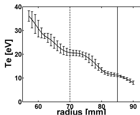
Figure 2. Radial profile of the electron temperature at the edge of CASTOR.
