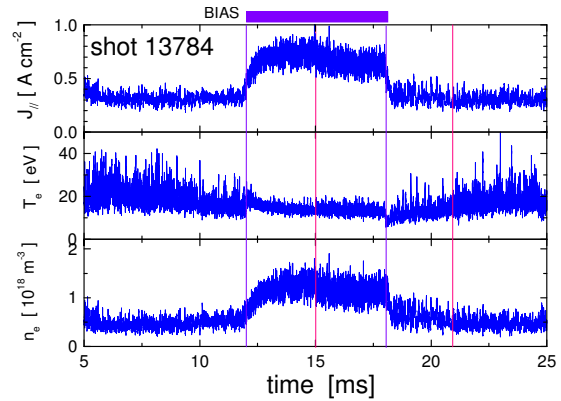
Figure 10. Temporal evolution of parallel current density J_{||} , the electron temperature and density during a shot with plasma biasing.
