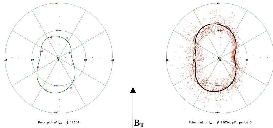
Fig. 3. Polar diagrams of the ion saturation current as measured in the same shot by the IGP (left) and the RMP (right) located inside the separatrix ( r= 70 mm). The experimental points are fitted to the KD model [2] (solid lines). #11054 .
