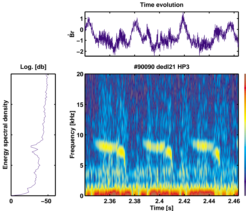
Figure 3. Record of sawtooth precursors..
