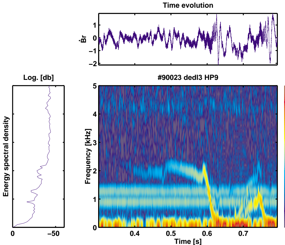
Figure 2. Time-frequency plot of B_r signal during disruption.
