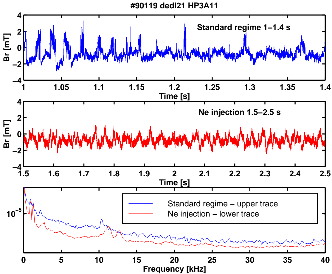
Figure 4. Suppression of magnetic turbulence over the whole spectrum in RI mode with energy feedback.
