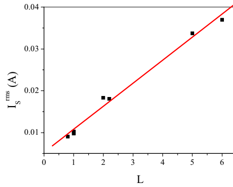
Fig. 3: The scaling factor versus the RMS of ion saturation current
