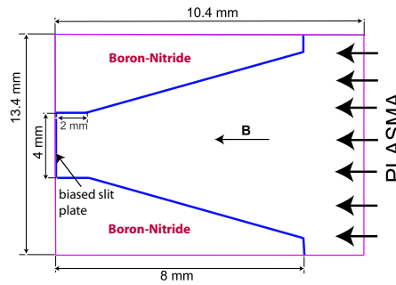
Fig. 5. XOOPIC model geometry.
