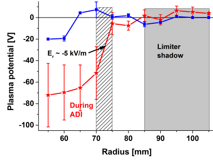
Figure 2: Radial profiles of the plasma potential during the appearance of the Anomalous Doppler Instability.
