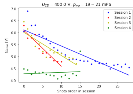
Figure 4: Evolution of the mean value of loop voltage during chosen sequence of discharges.
