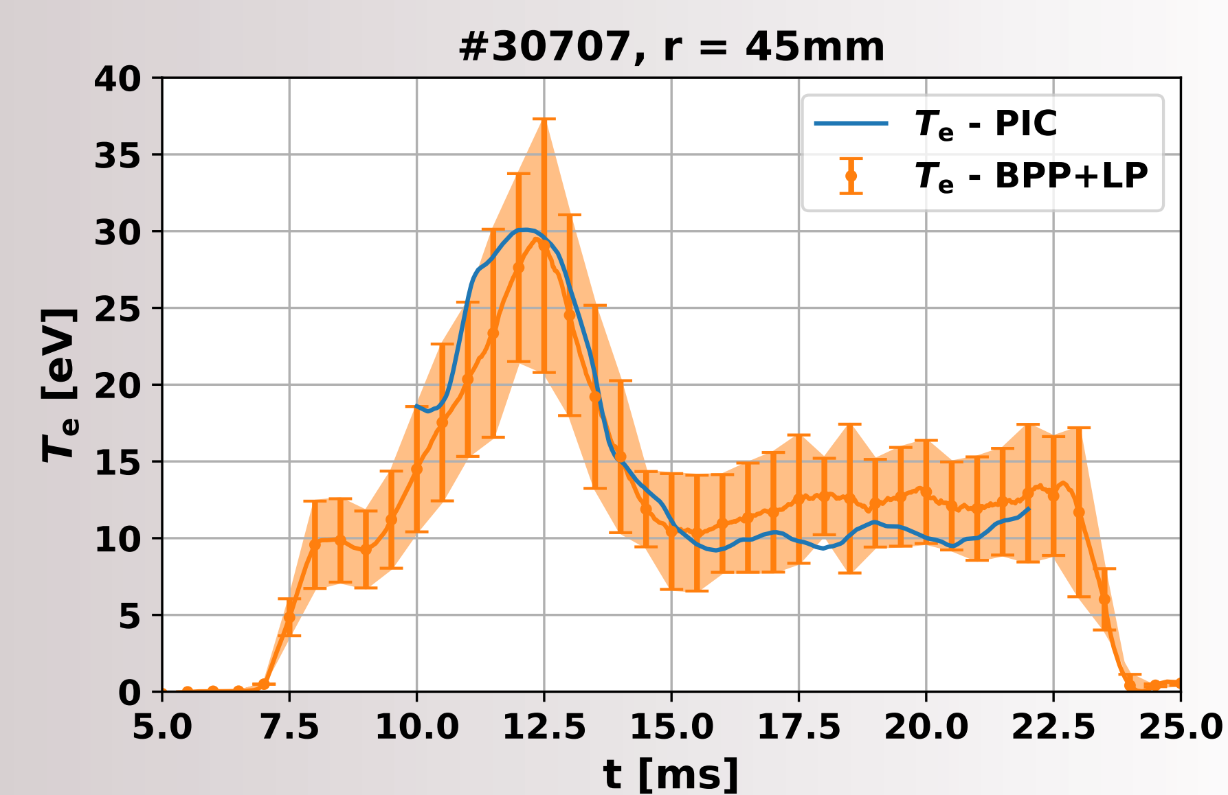
Time evolution of T_e measured by TP and BPP+LP.
