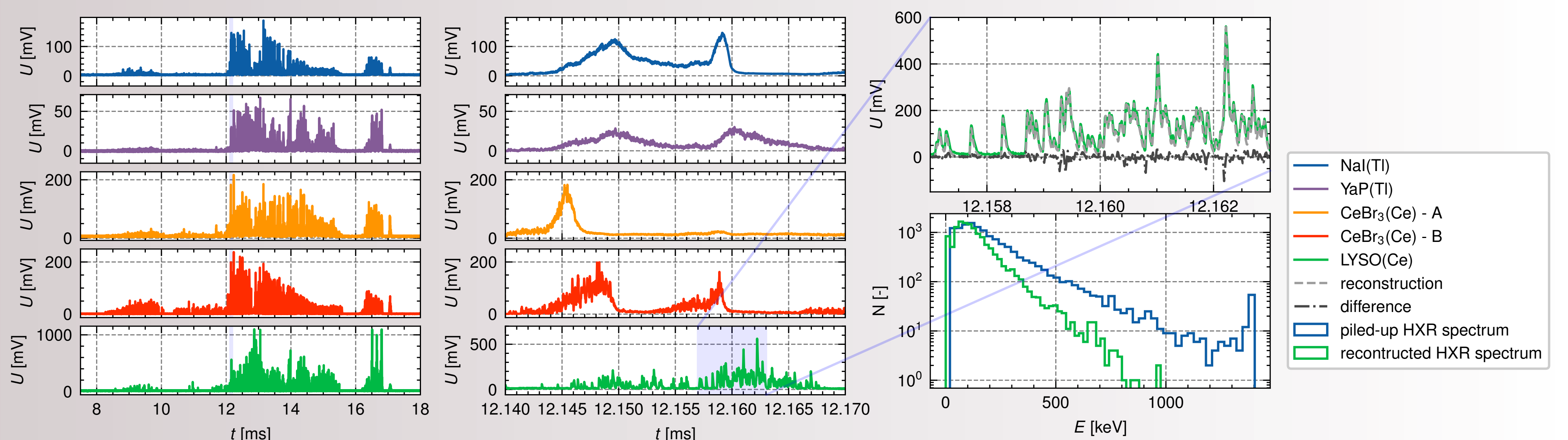
Left) Comparison of HXR signals from 5 scintillation detectors. Middle) More detailed plot. Right) HXR signal reconstruction, and corresponding spectrum.
