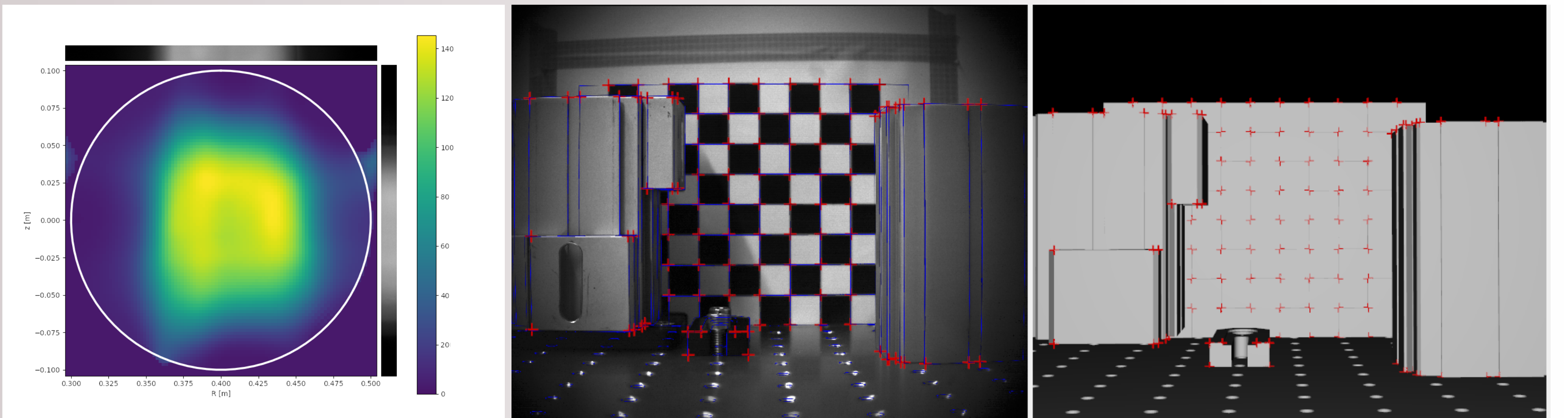
Left) preliminary tomographic reconstruction from discharge #39205, frame #231. White line represents the vessel wall, Right) camera lens calibration using Calcam software
