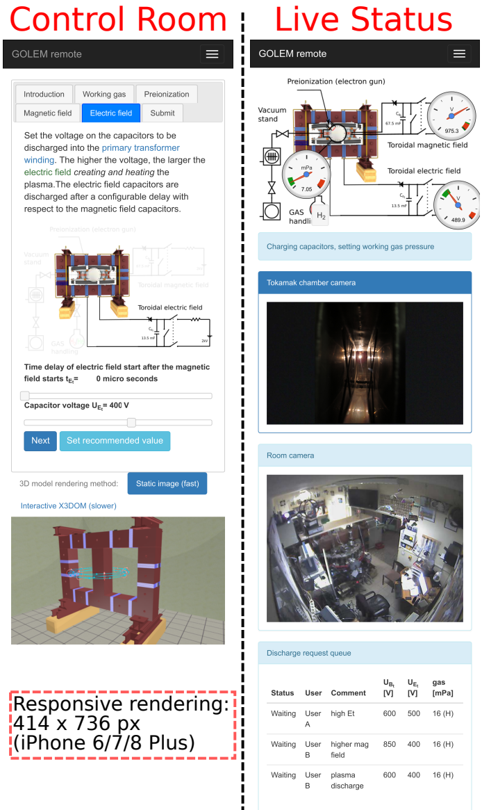
Fig. 1. Remote control and live status interface of the GOLEM tokamak as viewed on a mobile smartphone. The control room interface at the electric field setup step is shown on the left. The live real-time view of the experiment during the preparatory phase of the discharge is shown on the right.
