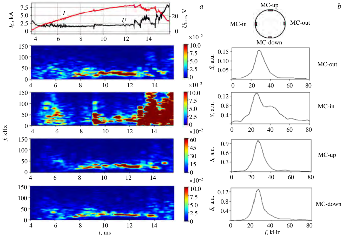
Fig. 24. Power spectrograms, H № 33 087 (a) and time-averaged (10 ms < t < 12.5 ms) power spectra (b) of the Mirnov Coil signals. Coherent magnetic fluctuation is excited in the range 20—40 kHz
