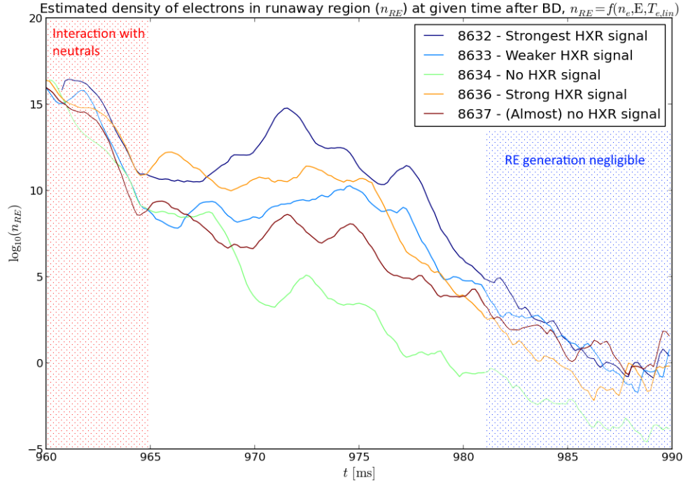
Figure 4.6: Analytical estimation of number of electrons in runaway region in the beginning of the discharge. The same linear increase of temperature and Z_{eff} = 2.5 is assumed for all discharges, however this assumptions change only the absolute value and not the relative differences between the curves. The comments on HXR intensity in the legend are related to the flat-top of the discharge. The intensity of HXR in the flat-top seems to be very well correlated to the estimated number. The regions that seem not be crucial for RE electron generation are dashed.
