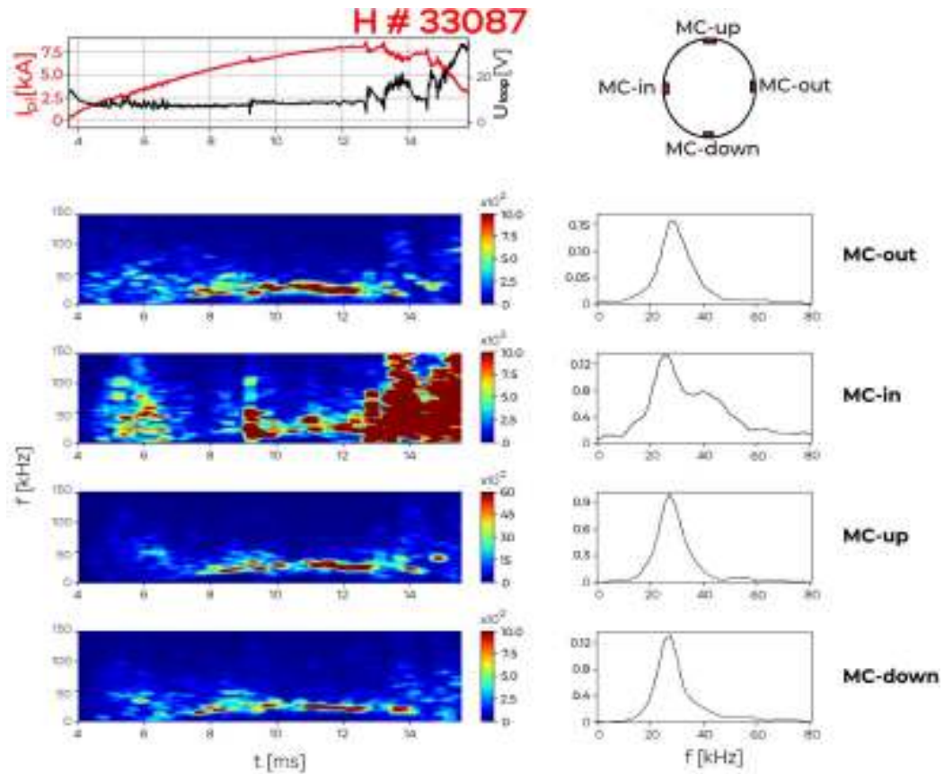
Figure 24. Power spectrograms (left) and time-averaged (10 ms < t < 12.5 ms) power spectra (right) of the Mirnov Coil signals. Coherent magnetic fluctuation is excited in the range 20-40 kHz.
