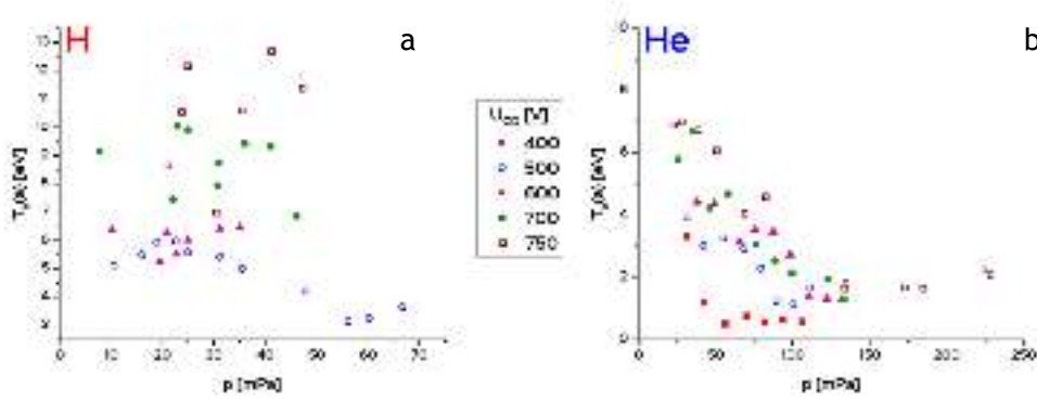
Figure 12. Edge electron temperature dependencies on initial gas pressure and current drive voltage at the moment of maximum plasma current in (a) hydrogen (b) helium discharge
