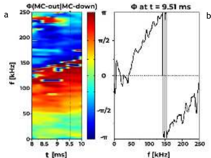
Fig.27. Cross-phase spectrogram of MC-out |MC-down signals (a) and cross-phase spectrum for t=9.51 \text{ ms} (b), shot #33052
