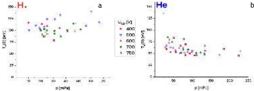
Figure 10. Dependence of the central electron temperature on the pressure for different current drive voltage in hydrogen (a) and helium (b) discharges
