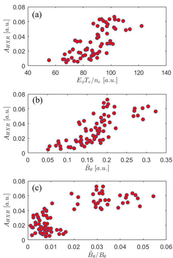
Figure 1. HXR signal amplitude ( A_{HXR} ) shows linear dependence on (a) normalized electric field ( E_\phi T_e / n_e ) (b) magnetic fluctuations ( \tilde{B}_\theta ) amplitude and (c) \tilde{B}_\theta / B_\theta .
