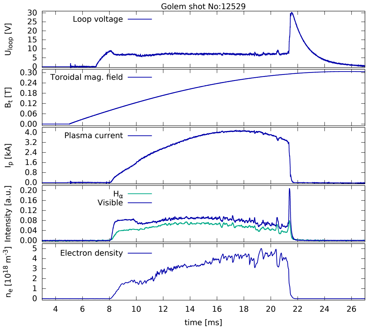
Figure 1: Evolution of a well executed GOLEM discharge. From top to bottom - the loop voltage U_{loop} , toroidal magnetic field B_t , plasma current I_p , the signal of photo-diode with H_\alpha interference filter and electron density n_e .
