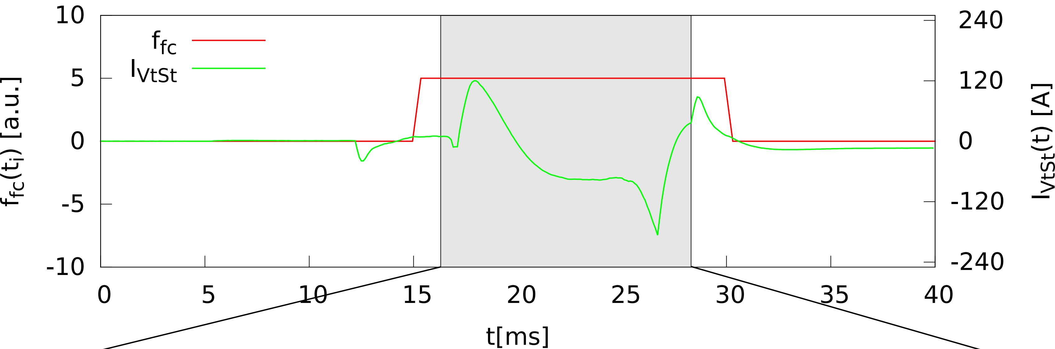
Feedback coefficient waveform & stabilization current for #16853
