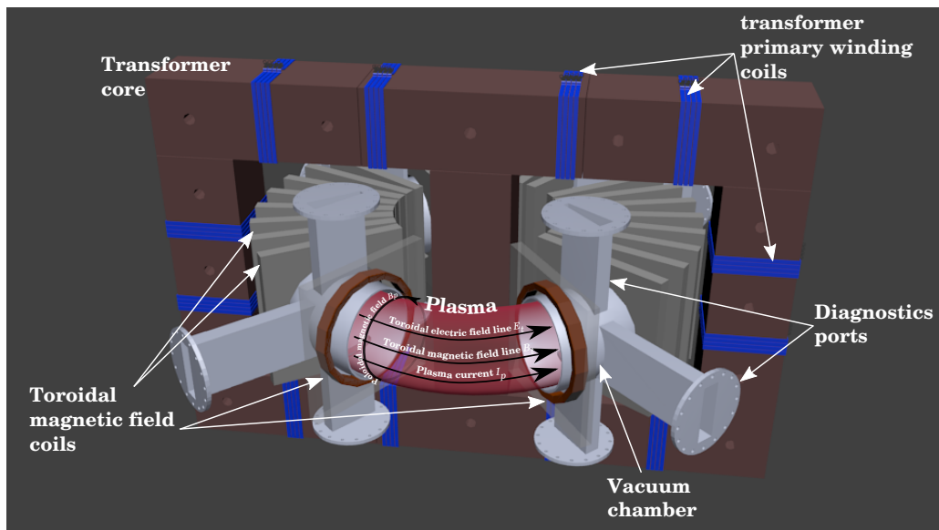
Figure 1: Tokamak (GOLEM) basic concept
