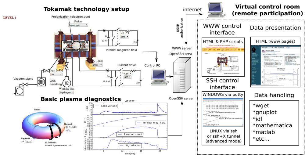
Figure 1: The global schematic overview of the tokamak GOLEM experiment
