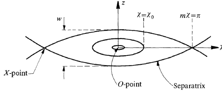
Figure 2.2: Characteristic local structure of perturbed B_\theta i.e. poloidal projection of magnetic island [4].
