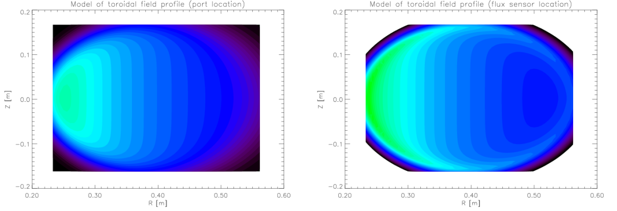
Figure 3.8: Model of B_T profile across the whole poloidal cross-section.
