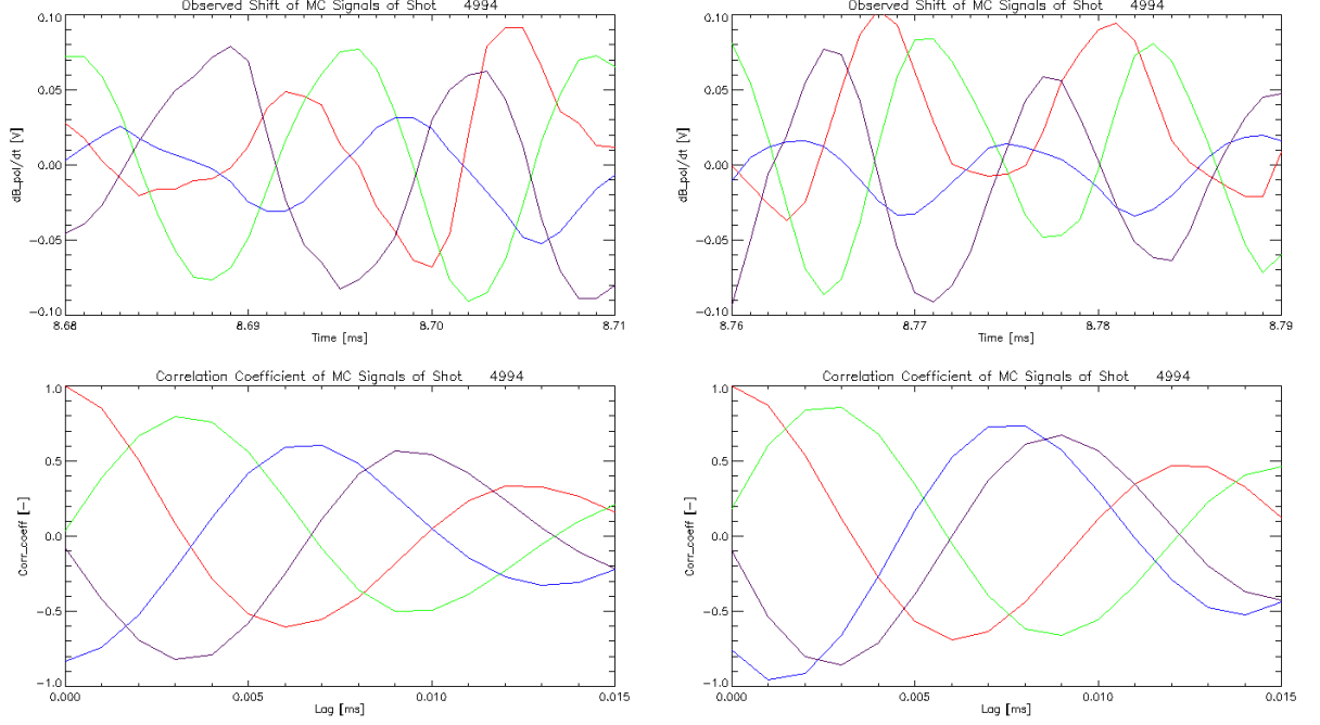
Figure 4.8: High sampling rate comparison of MC signals during initial current rise instabilities of shot 4994 (above), and their resultant correlation coefficients (calculated across the whole depicted evolution) with respect to MC01 (below). Red – MC01, green – MC05, blue – MC09, purple – MC13.
