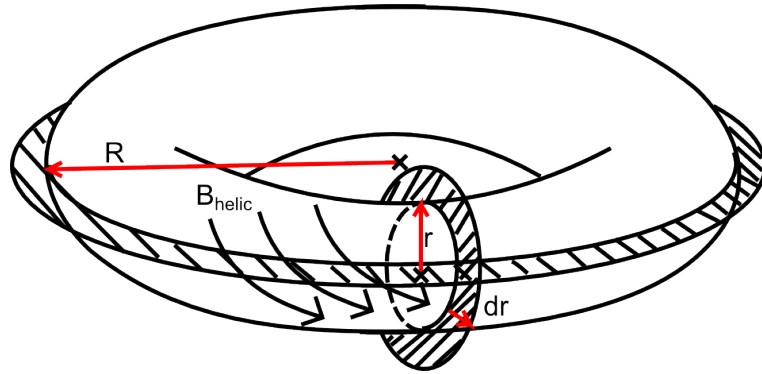
Figure 2.8: Geometry of q profile analysis for high aspect ratio tokamak of circular cross section.
