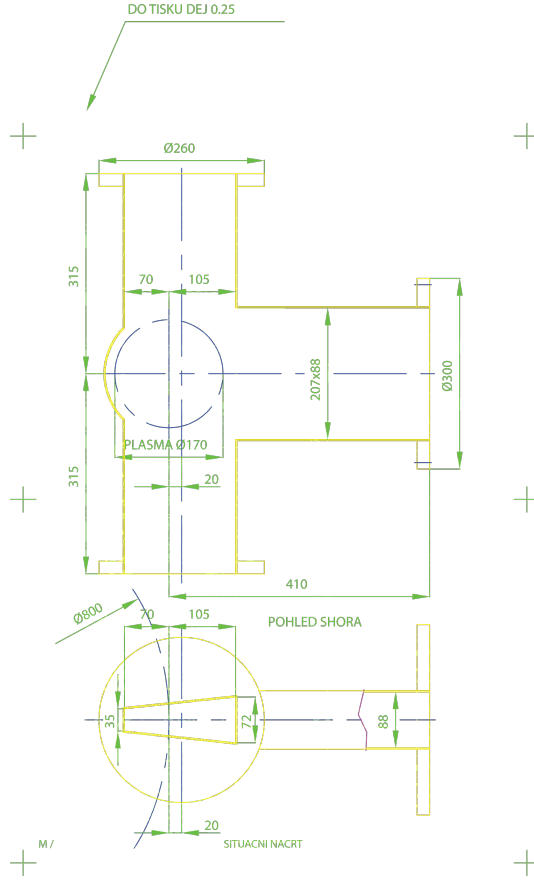
Figure 3.2: Blueprints of sets of large GOLEM diagnostic ports (in Czech).
