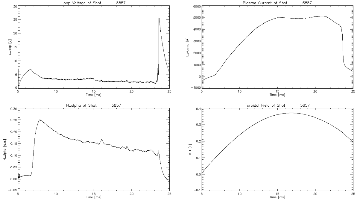
Figure 3.4: Typical evolutions of basic GOLEM discharge parameters (with passive stabilisation turned on in 15 th ms).
