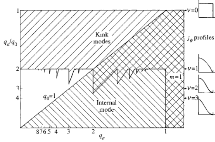
Figure 2.7: Combined stability diagram of constraints on q profile found in refs. [4] and [7].
