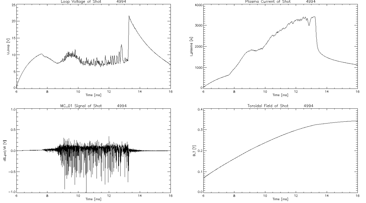
Figure 4.6: Plot of typical relevant parameters of small limiter GOLEM discharges.
