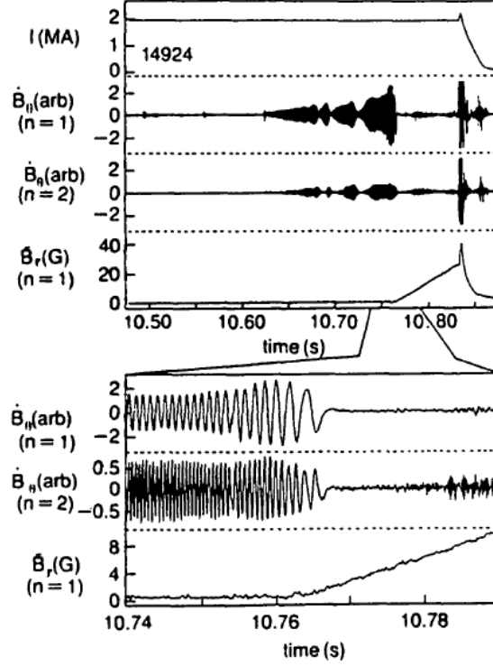
Figure 2.5: Idealized high density disruption of shot no. 14924 on JET tokamak from the viewpoint of global magnetic field parameters [2].
