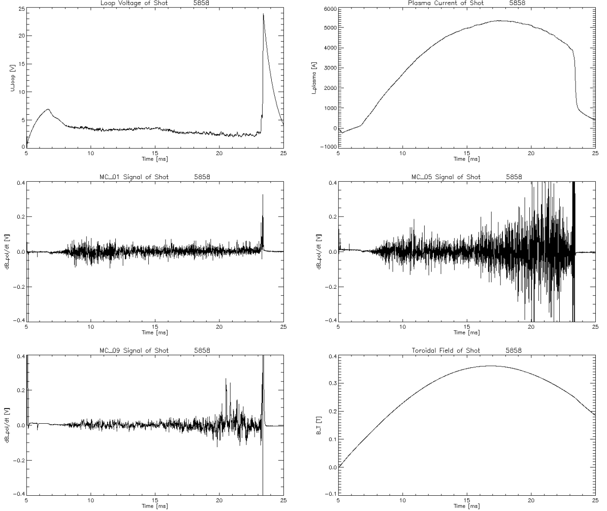
Figure 4.4: Plot of typical relevant parameters of stable shot with passive stabilisation turned on at 15 th ms.
