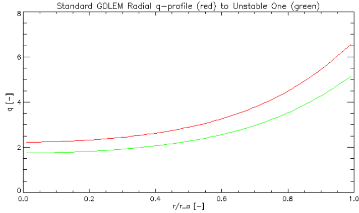
Figure 4.1: Radial q -profiles for standard GOLEM operational parameters of B_T = 0.37 T, I_p = 5 kA, a_1 = 0.085 m (red), and for parameters of small limiter discharge B_T = 0.35 T, I_p = 3 kA, a_2 = 0.060 m (green) given that \nu = 2 in both cases.
