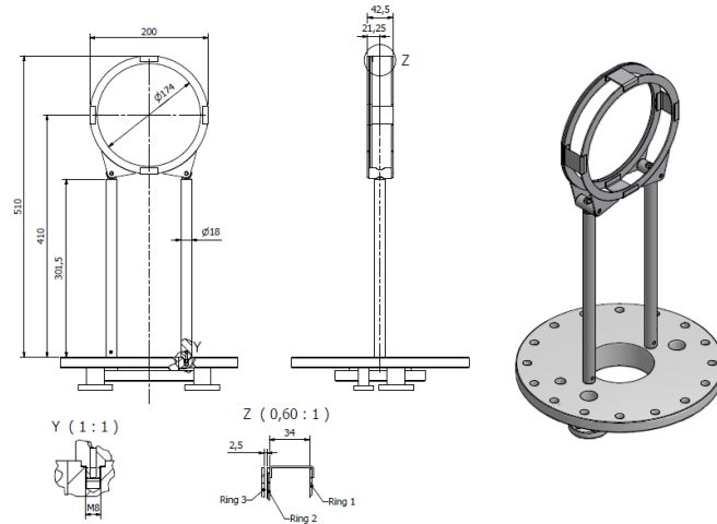
Figure 3.13: Final blueprints of new support construction for new set of 16 Mirnov coils and 4 3D Hall probes (made by Vakuum Praha ).
