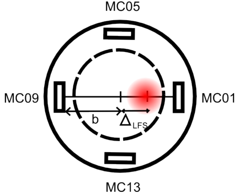
Figure 3.11: Spatial distribution and notation of available Mirnov coils (MCs) across the whole poloidal circumference.
