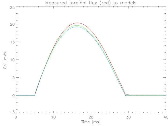
Figure 3.12: Comparison of measured total toroidal flux \chi (red line) to model by Biot-Savart (green line) and by Ampere (blue line).
