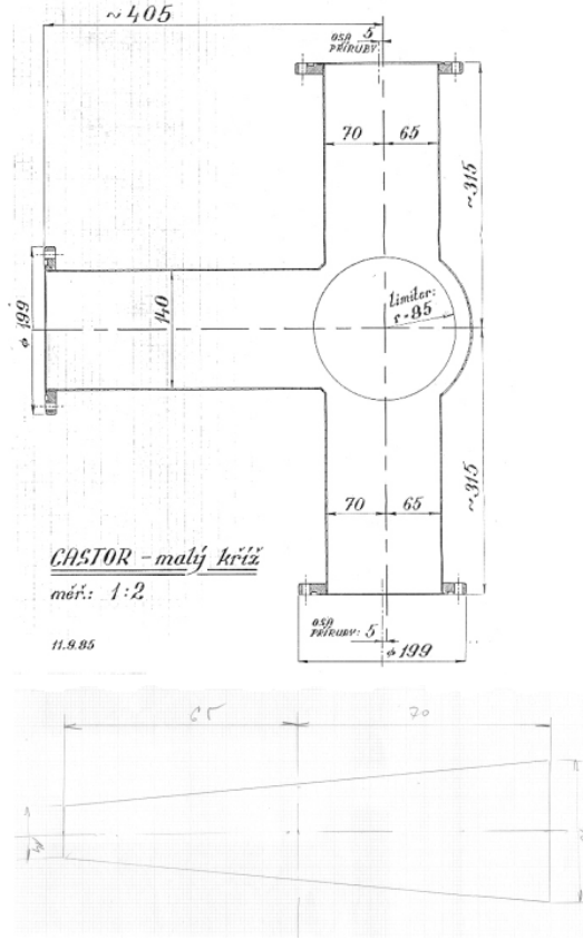
Figure 3.3: Blueprints of sets of small GOLEM diagnostic ports (in Czech). View from above is included in the lower part of the figure.
