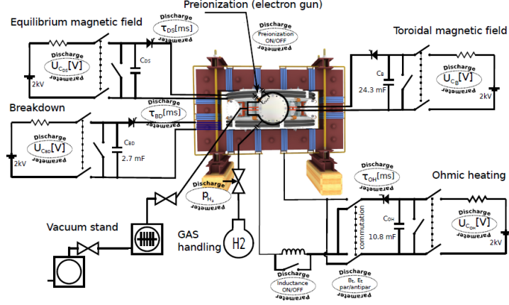
Figure 3.5: Engineering scheme of tokamak GOLEM with respective control parameters. Taken from ref. [14].
