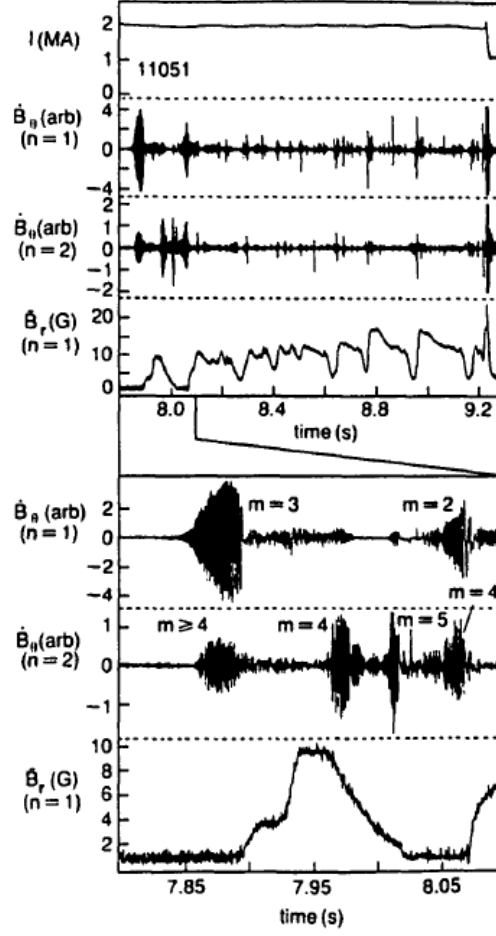
Figure 2.6: Standard high density disruption of shot no. 11051 on JET tokamak from the viewpoint of global magnetic field parameters [2].
