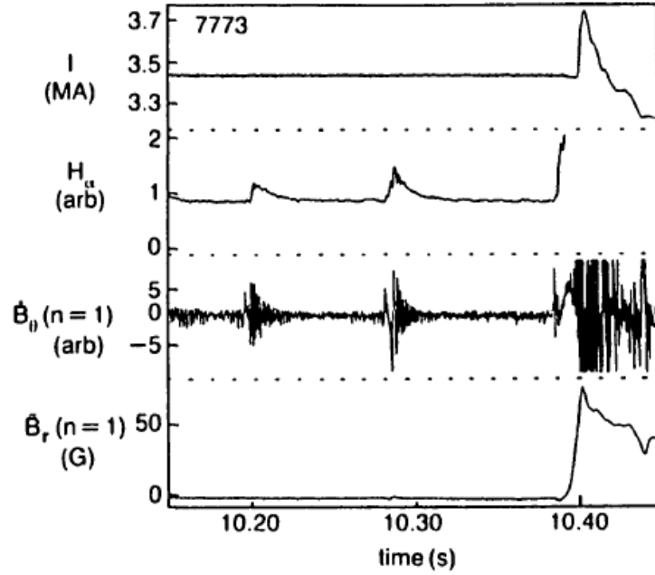
Figure 2.4: Low q disruption of shot no. 7773 on JET tokamak from the viewpoint of global tokamak parameters with sawteeth present [2].
