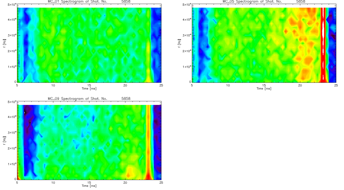
Figure 4.5: Frequency spectra of \dot{B}_\theta signal fluctuations detected by respective MCs.
