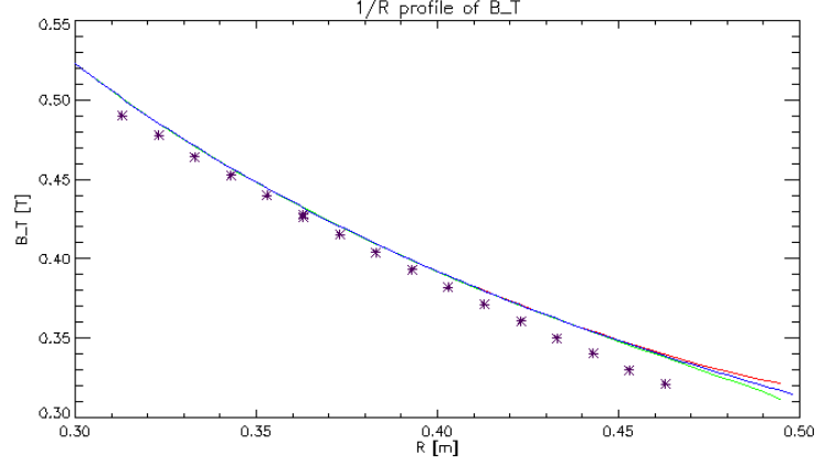
Figure 3.9: B_T field 1/R profile at Z = 0 (i.e. central midplane) with R limited by liner dimensions. All the magnitudes correspond to 3500 A peak of B_T capacitors discharge current output and thus represent typical magnitudes of GOLEM discharge. Blue line represents 1/R of Ampere's law, green line profile on the left in fig. 3.8, red line profile on the right in fig. 3.8 and purple asterisks directly measured values by 3D Hall probe.
