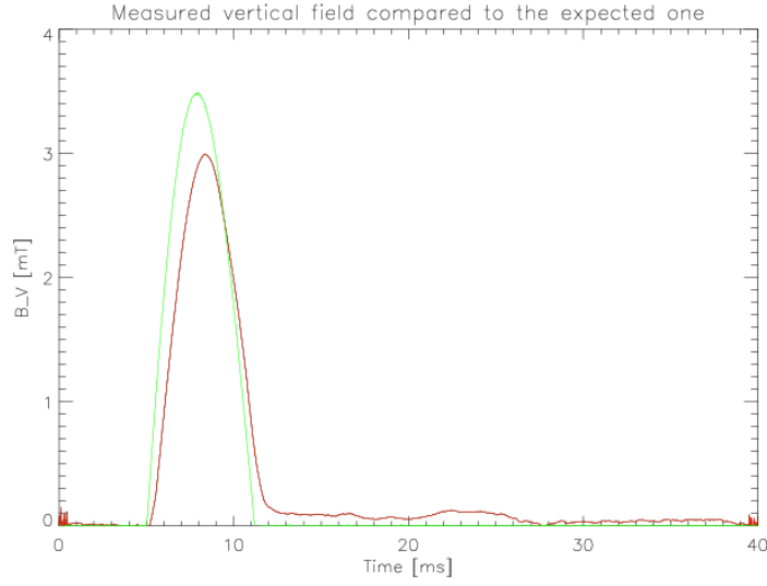
Figure 3.7: Comparison of measured magnitude of B_V generated by inner stabilisation coils (red line) to values given by application of Biot-Savart's law on their spatial configuration and currents (green line).
