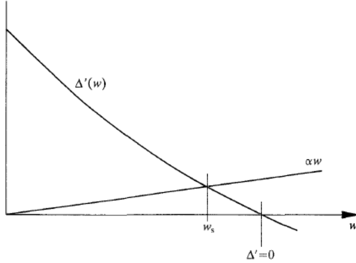
Figure 2.9: Evolutions of w -dependant terms of eq. 2.39 [4], implying stability of saturated width w_s .
