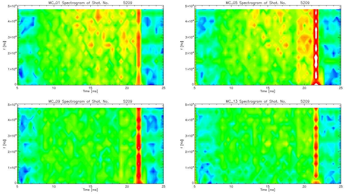
Figure 4.3: Frequency spectra of \dot{B}_\theta signal fluctuations detected by respective MCs.
