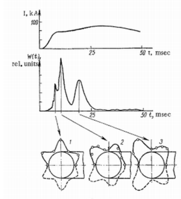
Figure 2.10: Relation of magnetic field oscillations to plasma current as observed in ref. [13]. Please note that w quantity here does not represent island width but magnitude of B_\theta perturbations (although these two quantities strongly correlate with each other).
