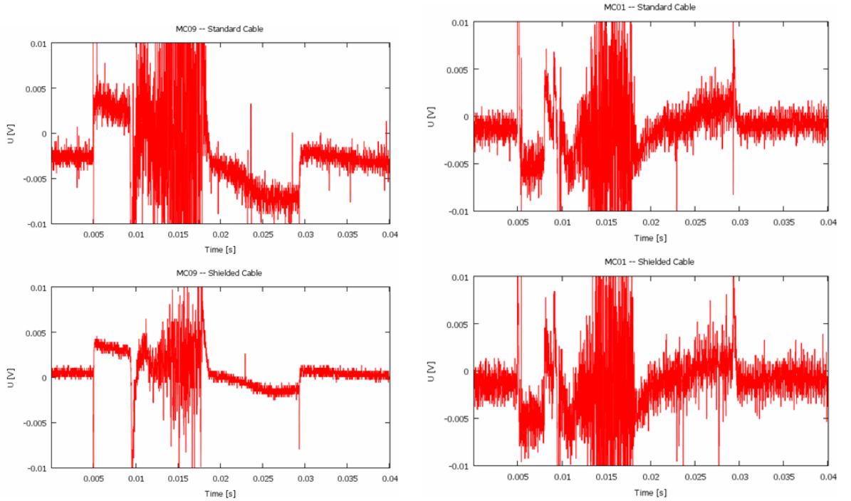
Figure 3.10: Two essentially same signals of B_T cross-talk and plasma signal on Mirnov coil 9 (HFS location) and Mirnov coil 1 (LFS location) acquired by different cables.
