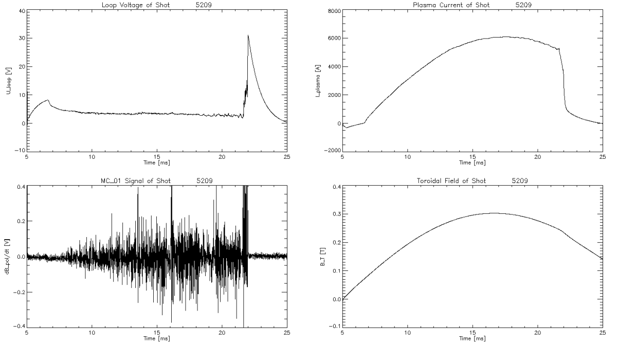
Figure 4.2: Plot of typical relevant parameters of stable shot without passive stabilisation enabled.
