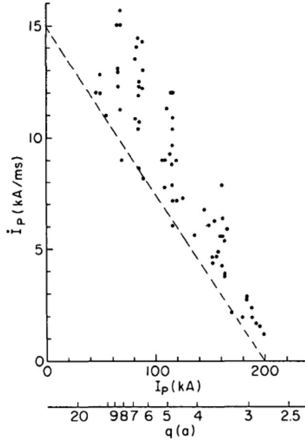
Figure 2.3: Emergence of current rise disruptions on Alcator A tokamak with dependance on global plasma parameters [6].
