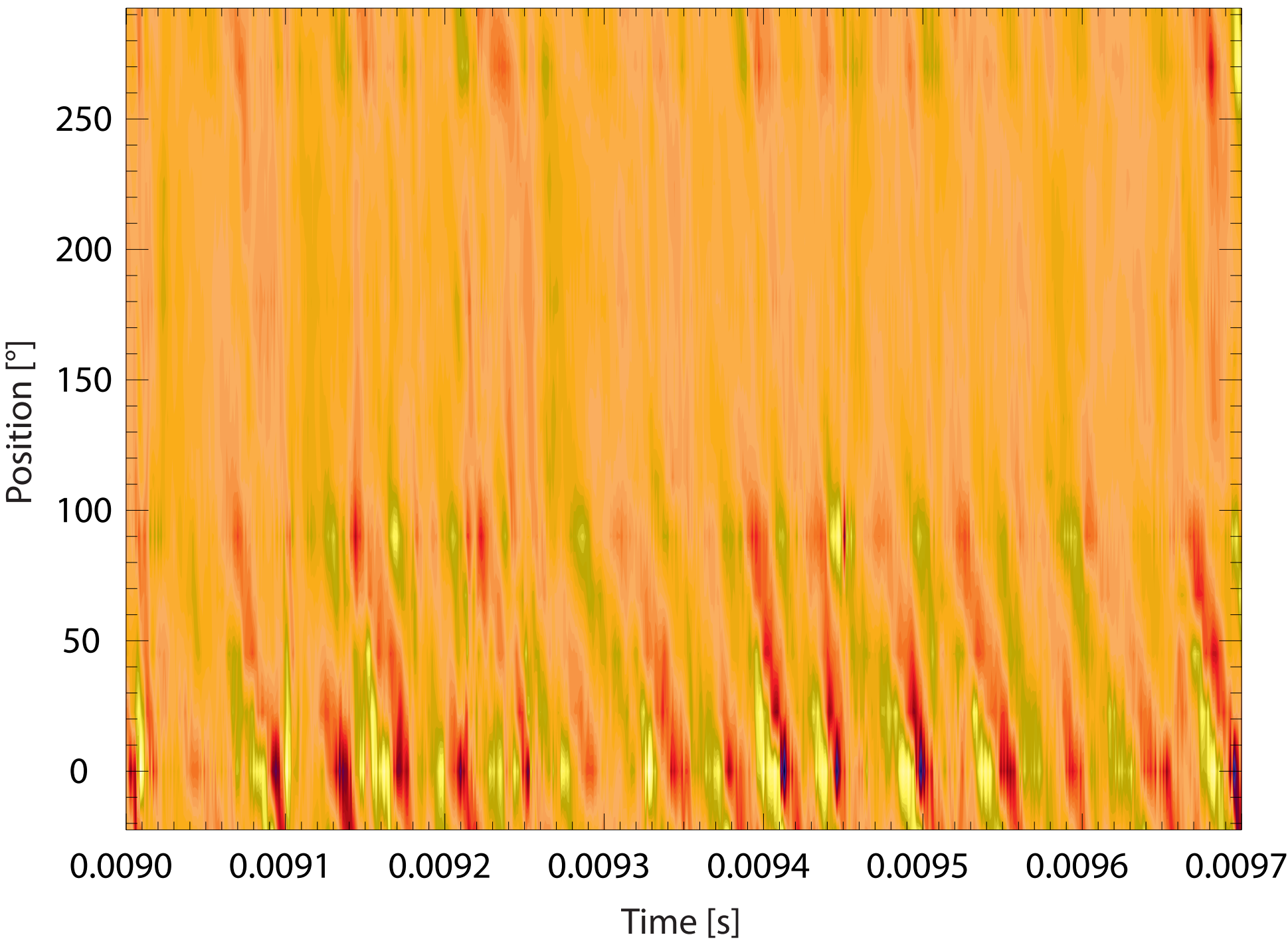
Signal of the new magnetic coils in shot 8253
