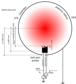
Ball-pen probe
