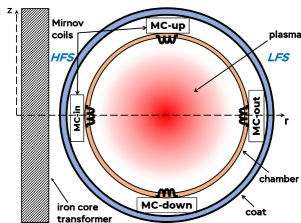
Mirnov coils to measure MHD activity
