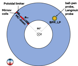
Experimental set-up
