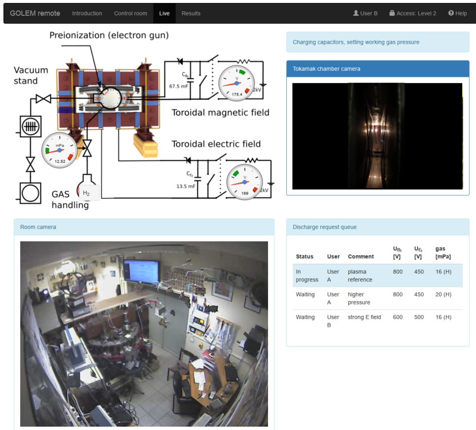
Figure 1: Web page displaying the live real-time view of the experiment during the preparatory phase of the discharge. The gauges over the engineering scheme (top left) show the gradual charging of capacitors and filling of the chamber with the selected working gas. The room camera (bottom left) shows the general surroundings of the device, while the chamber camera (top right) shows the pre-ionization filament activation. The queue of discharge requests with the most important basic parameters is shown in the bottom right.
