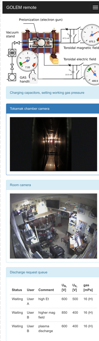
Fig. 1. Remote control and live status interface of the GOLEM tokamak as viewed on a mobile smartphone. The control room interface at the electric field setup step is shown on the left. The live real-time view of the experiment during the preparatory phase of the discharge is shown on the right.
